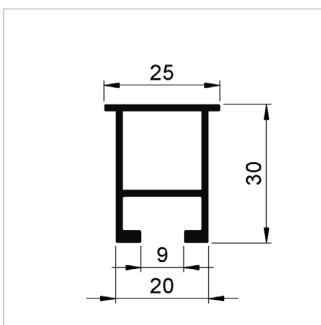
91B profile dimensions.
