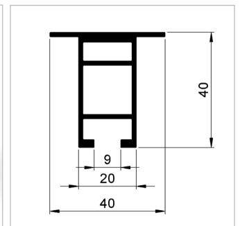
92B profile dimensions.
