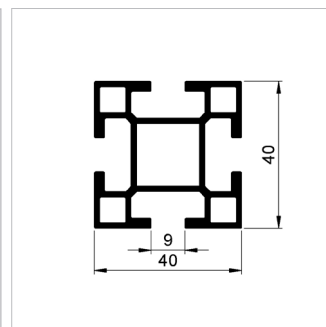
194 profile dimensions
