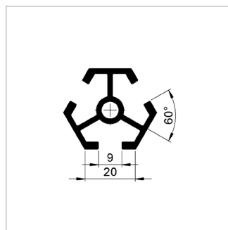
333 profile dimensions
