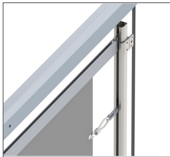
SMART-Lift has a very solid lift device with ball-mounted rollers running in an enclosed rail.
